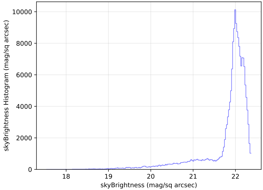
internal_u_expt60_nscale1.2v3.4_10yrs All sky g band: skyBrightness Histogram
