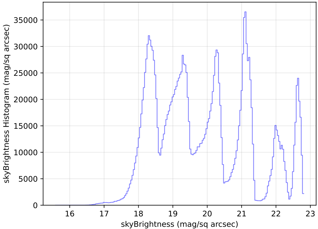
internal_u_expt60_nscale1.2v3.4_10yrs All sky all bands: skyBrightness Histogram
