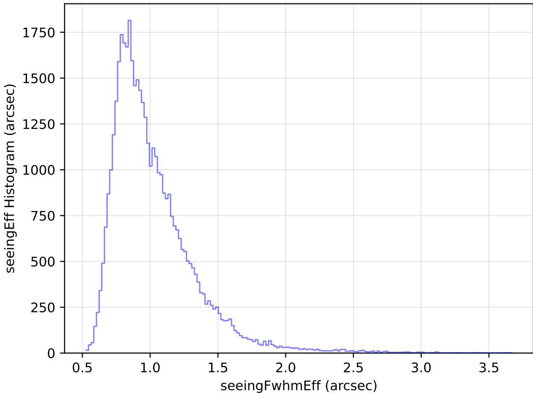
internal_u_expt60_nscale1.2v3.4_10yrs Yr 1 z band: seeingEff Histogram
