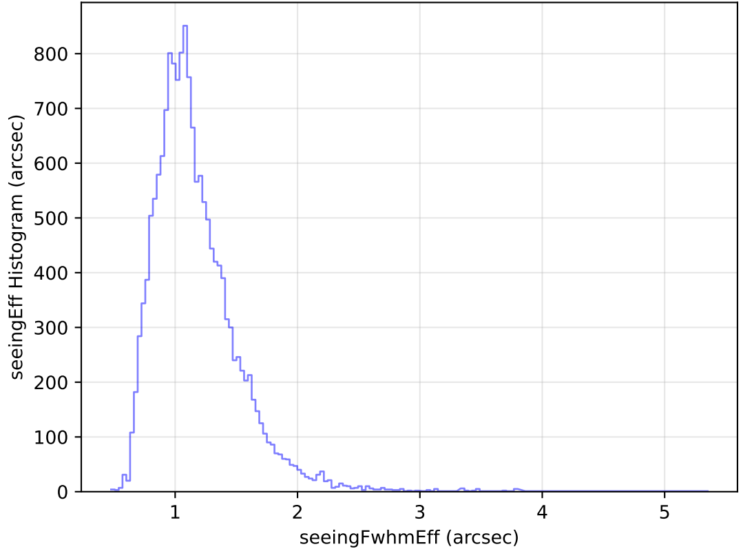
internal_u_expt60_nscale1.2v3.4_10yrs Yr 1 u band: seeingEff Histogram
