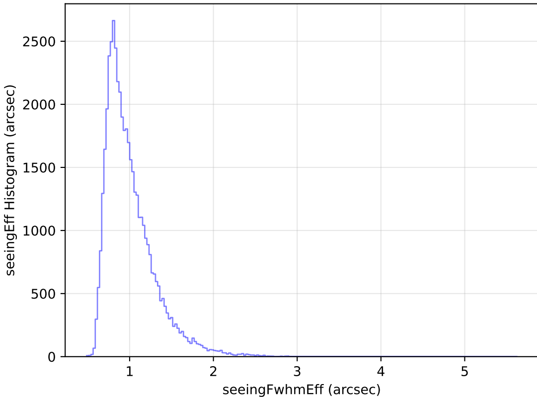
internal_u_expt60_nscale1.2v3.4_10yrs Yr 1 r band: seeingEff Histogram
