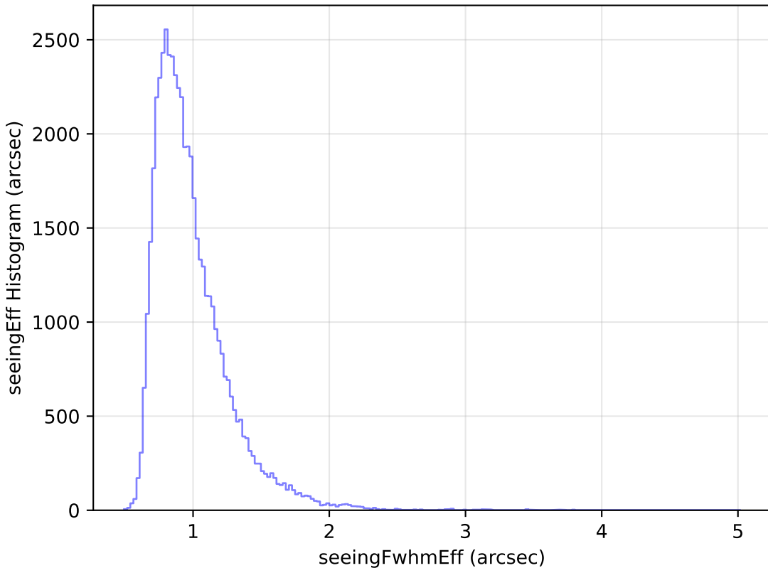
internal_u_expt60_nscale1.2v3.4_10yrs Yr 1 i band: seeingEff Histogram
