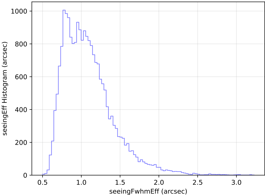
internal_u_expt60_nscale1.2v3.4_10yrs Yr 1 g band: seeingEff Histogram
