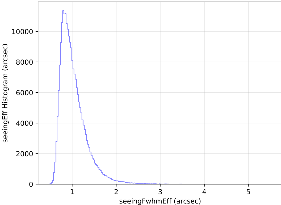
internal_u_expt60_nscale1.2v3.4_10yrs Yr 1 all bands: seeingEff Histogram
