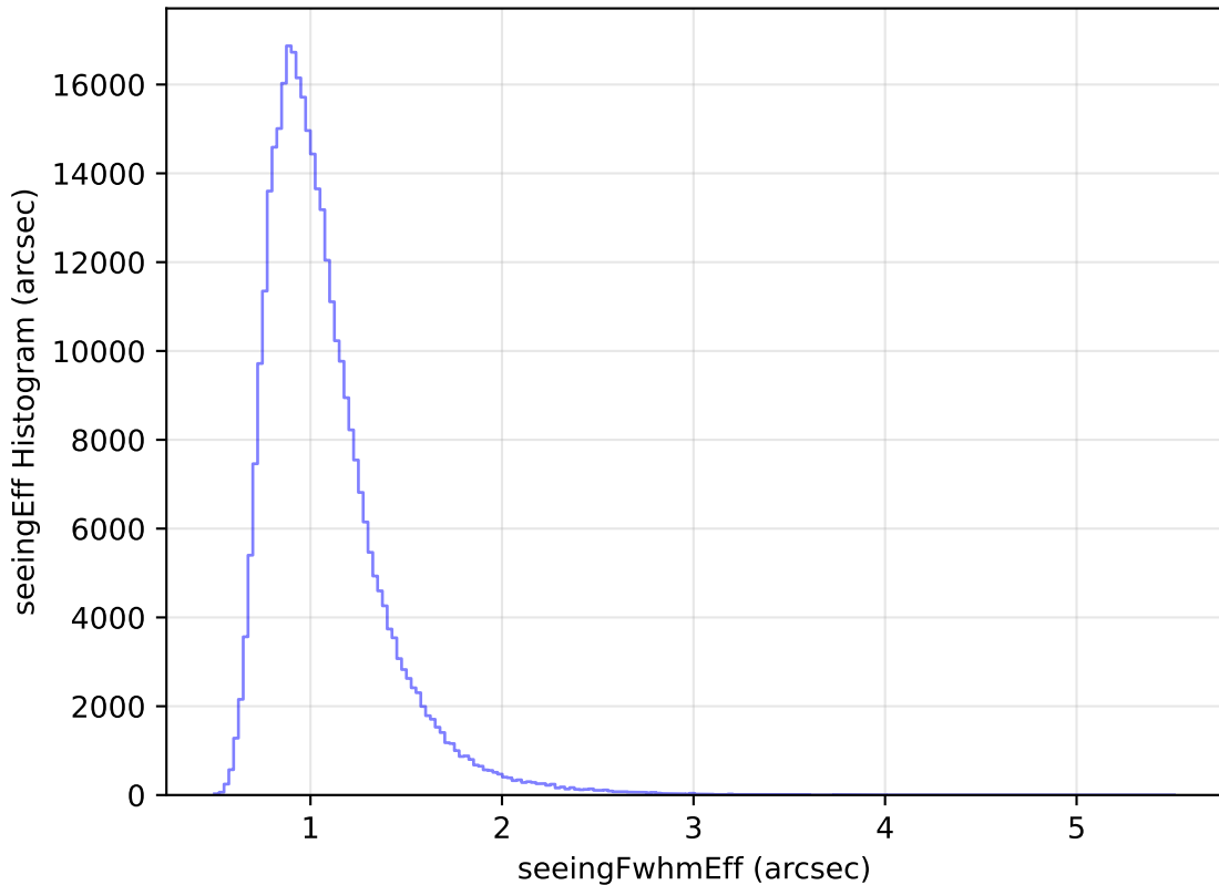
internal_u_expt60_nscale1.2v3.4_10yrs WFD y band: seeingEff Histogram
