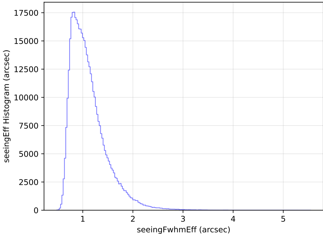
internal_u_expt60_nscale1.2v3.4_10yrs WFD r band: seeingEff Histogram
