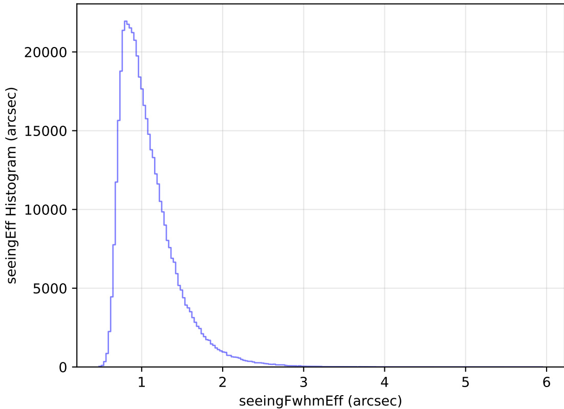
internal_u_expt60_nscale1.2v3.4_10yrs WFD i band: seeingEff Histogram
