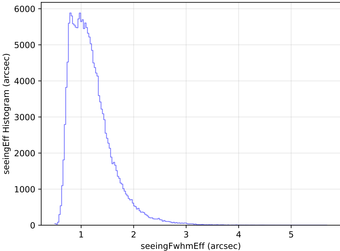
internal_u_expt60_nscale1.2v3.4_10yrs WFD g band: seeingEff Histogram
