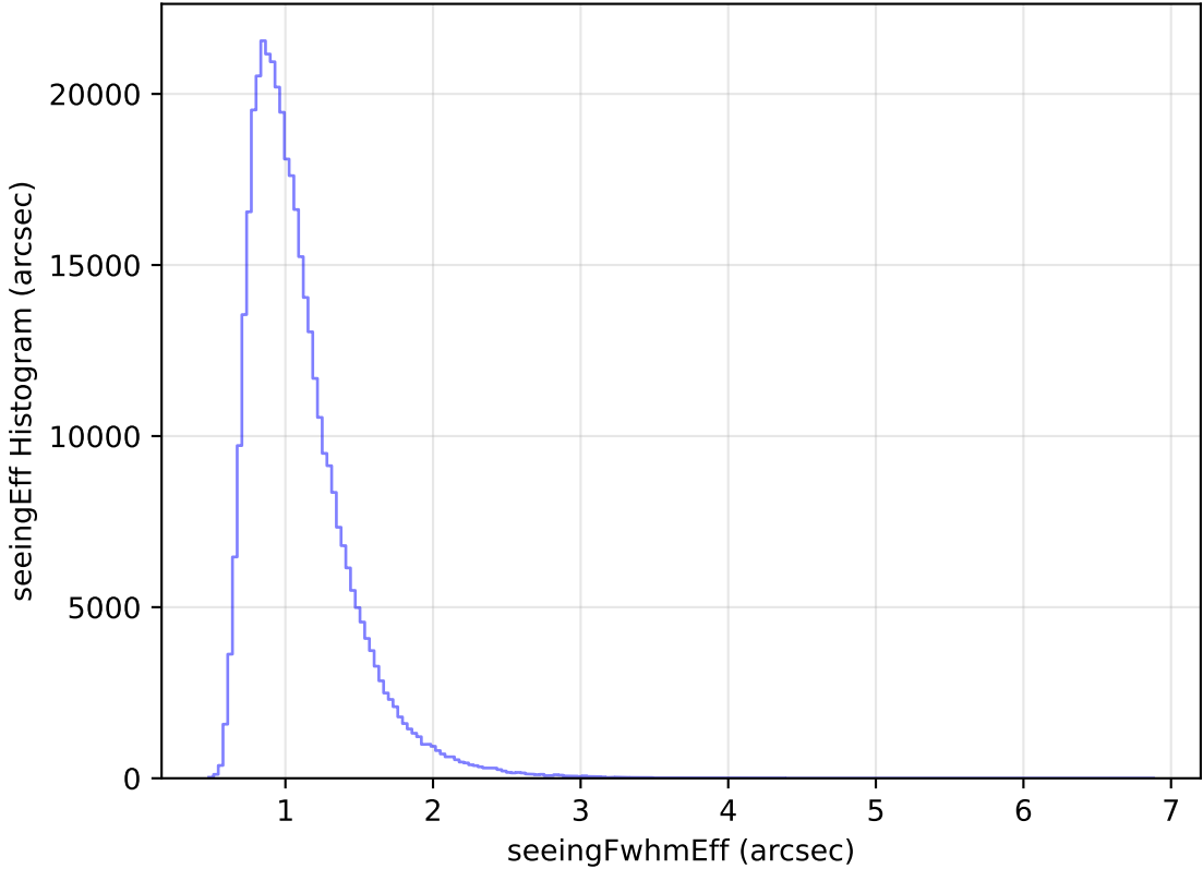
internal_u_expt60_nscale1.2v3.4_10yrs All sky z band: seeingEff Histogram
