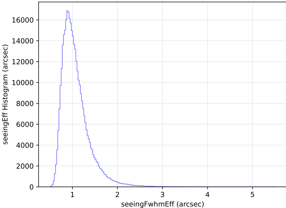
internal_u_expt60_nscale1.2v3.4_10yrs All sky y band: seeingEff Histogram
