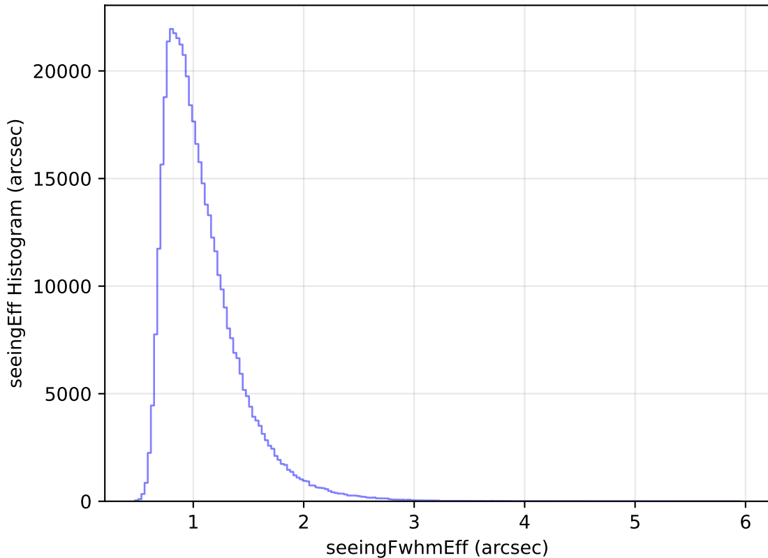
internal_u_expt60_nscale1.2v3.4_10yrs All sky i band: seeingEff Histogram
