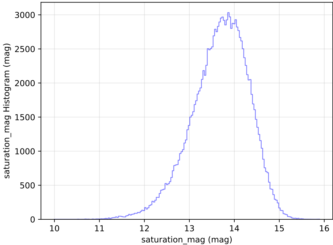
internal_u_expt60_nscale1.2v3.4_10yrs WFD u band: saturation_mag Histogram
