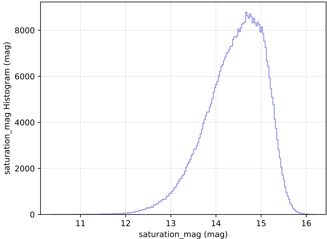
internal_u_expt60_nscale1.2v3.4_10yrs WFD i band: saturation_mag Histogram
