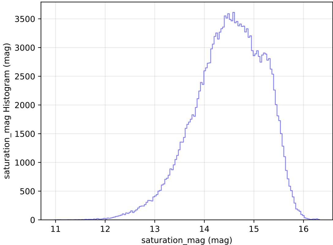
internal_u_expt60_nscale1.2v3.4_10yrs WFD g band: saturation_mag Histogram
