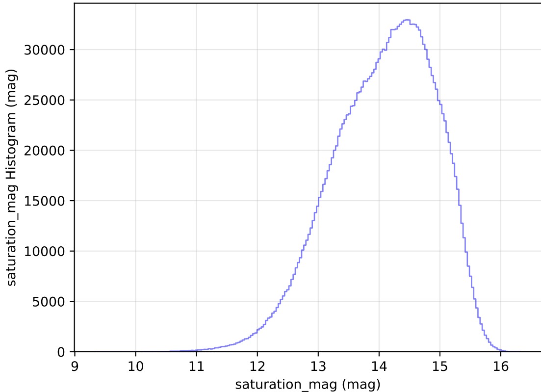
internal_u_expt60_nscale1.2v3.4_10yrs WFD all bands: saturation_mag Histogram
