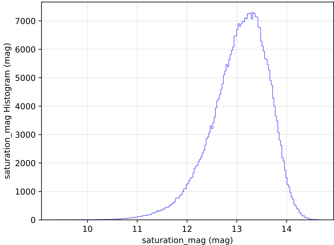
internal_u_expt60_nscale1.2v3.4_10yrs All sky y band: saturation_mag Histogram
