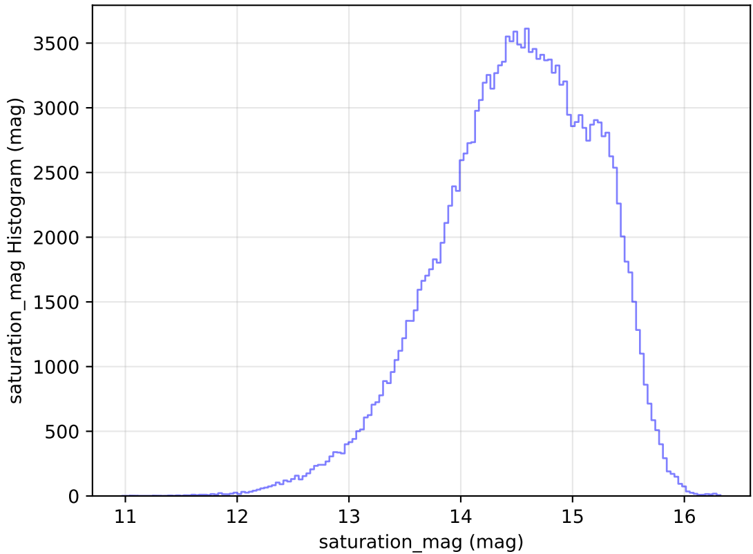
internal_u_expt60_nscale1.2v3.4_10yrs All sky g band: saturation_mag Histogram
