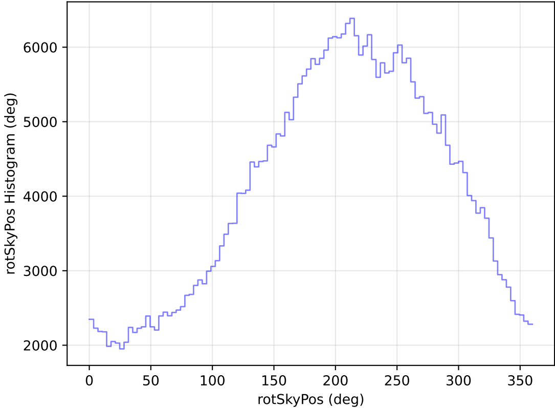
internal_u_expt60_nscale1.2v3.4_10yrs WFD z band: rotSkyPos Histogram
