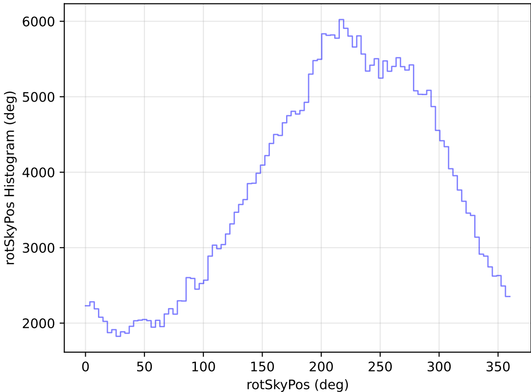
internal_u_expt60_nscale1.2v3.4_10yrs WFD y band: rotSkyPos Histogram
