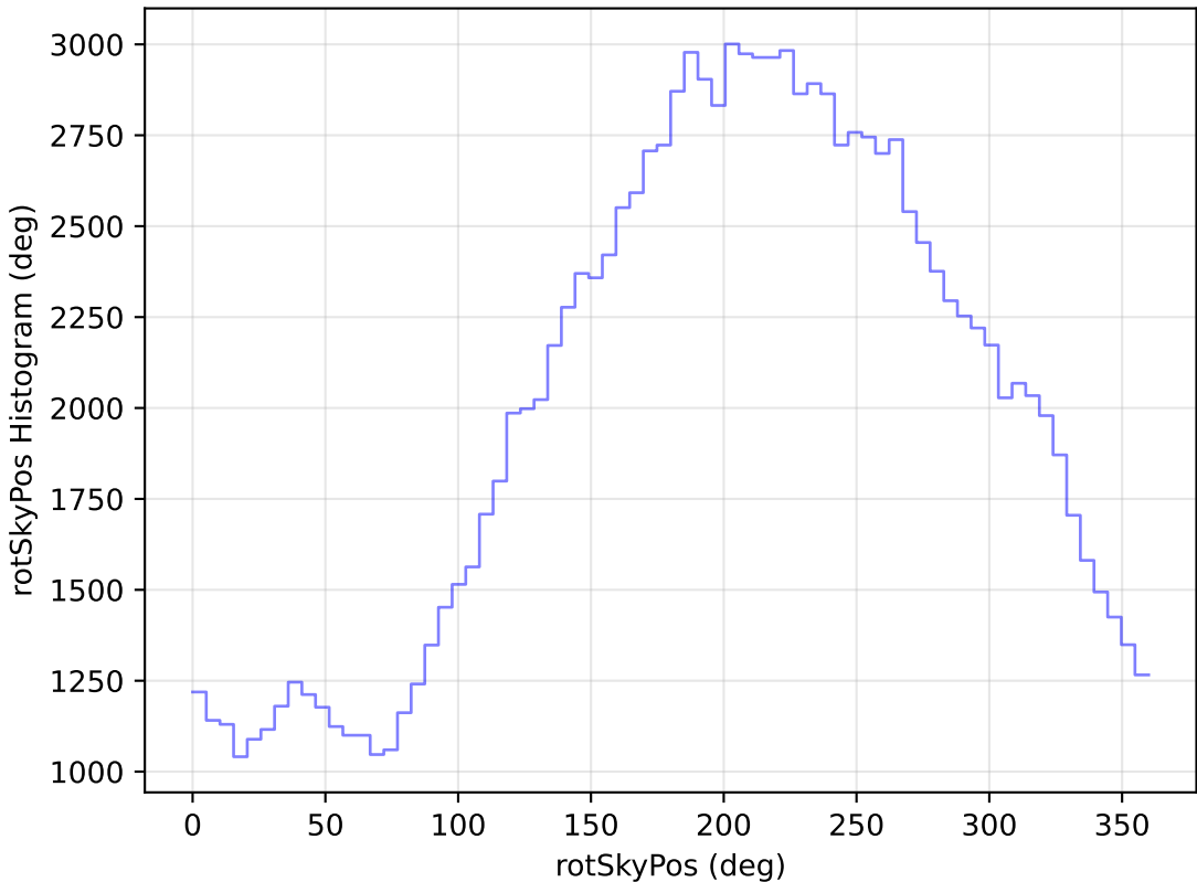
internal_u_expt60_nscale1.2v3.4_10yrs WFD u band: rotSkyPos Histogram
