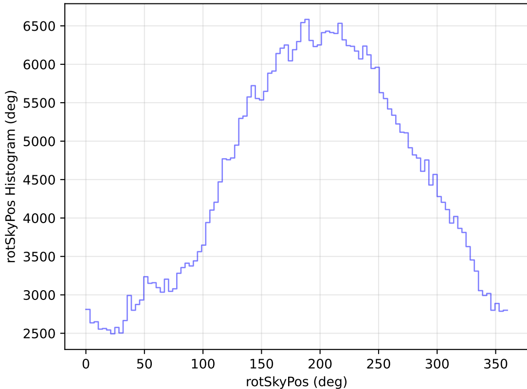
internal_u_expt60_nscale1.2v3.4_10yrs WFD r band: rotSkyPos Histogram
