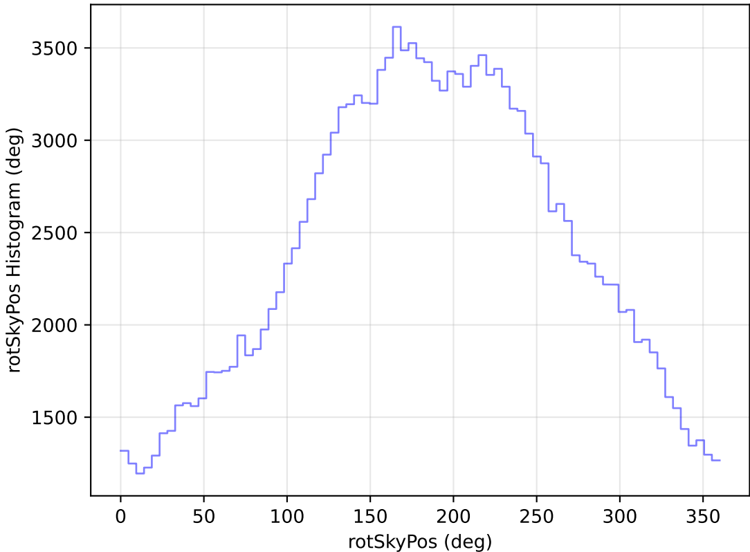
internal_u_expt60_nscale1.2v3.4_10yrs WFD g band: rotSkyPos Histogram
