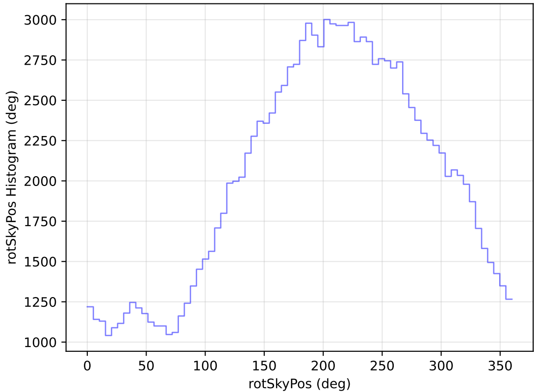
internal_u_expt60_nscale1.2v3.4_10yrs All sky u band: rotSkyPos Histogram
