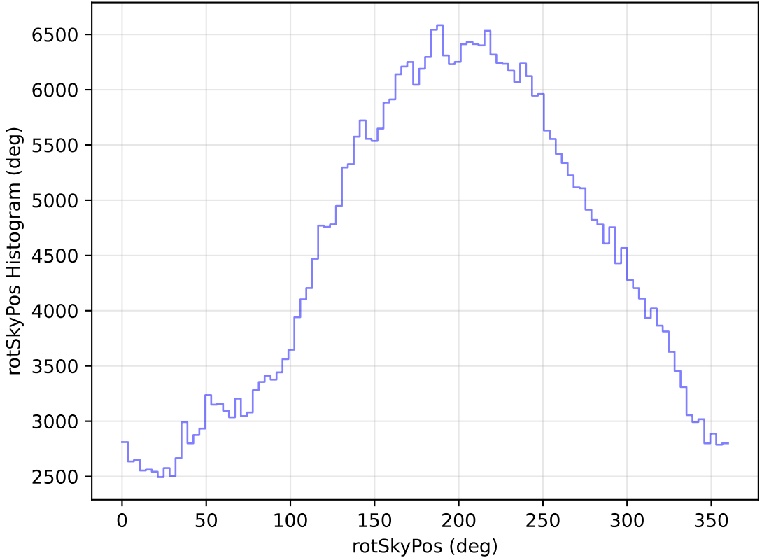
internal_u_expt60_nscale1.2v3.4_10yrs All sky r band: rotSkyPos Histogram
