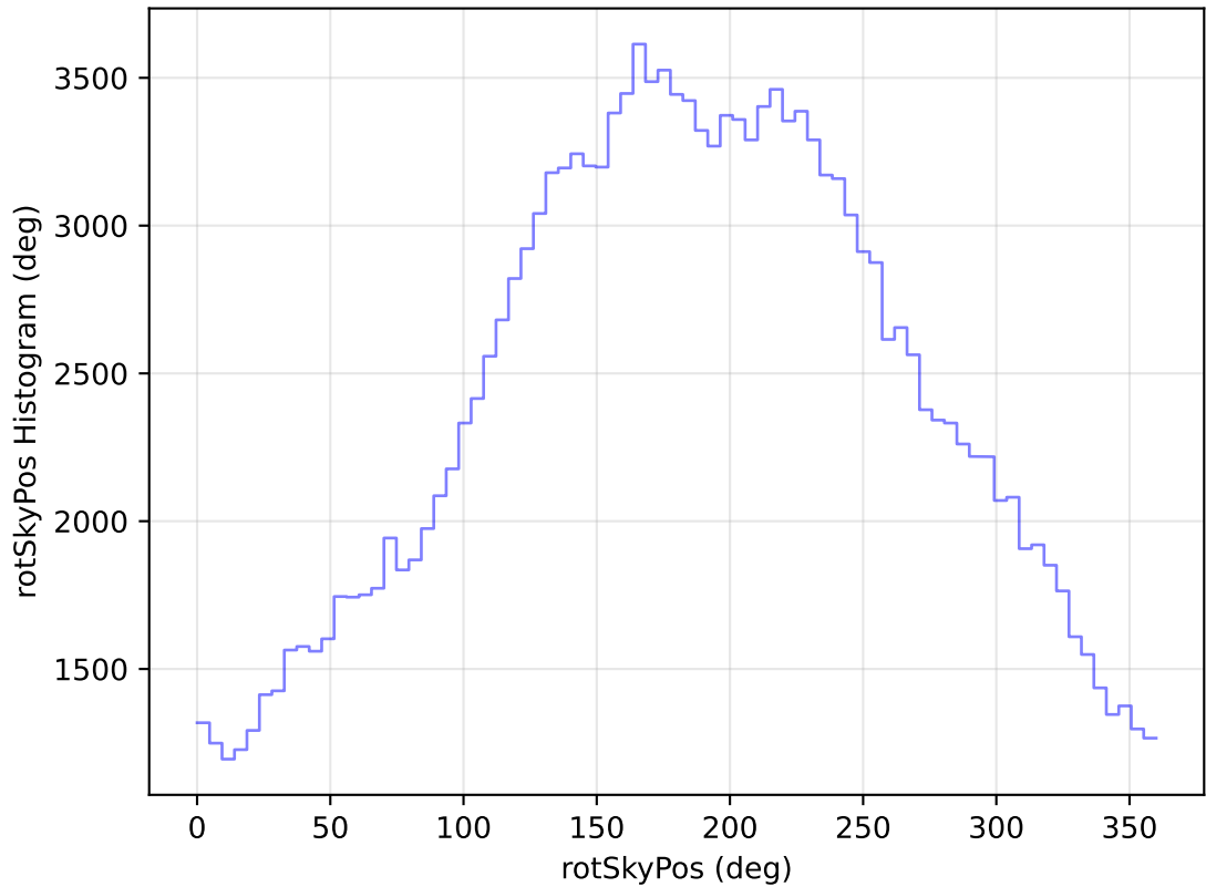
internal_u_expt60_nscale1.2v3.4_10yrs All sky g band: rotSkyPos Histogram
