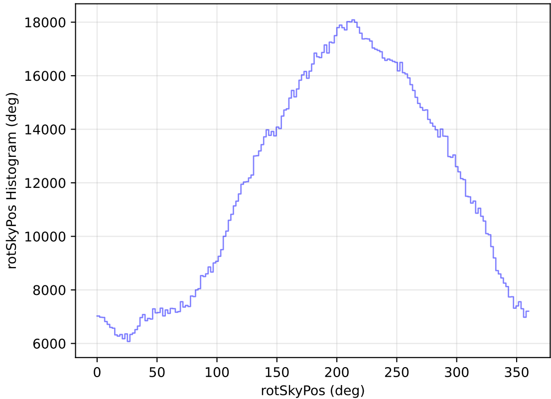
internal_u_expt60_nscale1.2v3.4_10yrs All sky all bands: rotSkyPos Histogram
