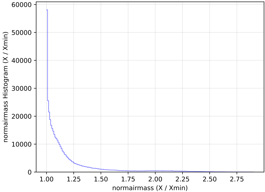
internal_u_expt60_nscale1.2v3.4_10yrs WFD z band: normairmass Histogram
