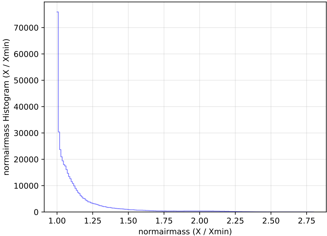
internal_u_expt60_nscale1.2v3.4_10yrs WFD r band: normairmass Histogram
