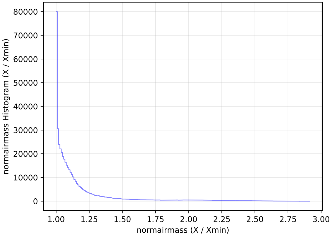
internal_u_expt60_nscale1.2v3.4_10yrs WFD i band: normairmass Histogram
