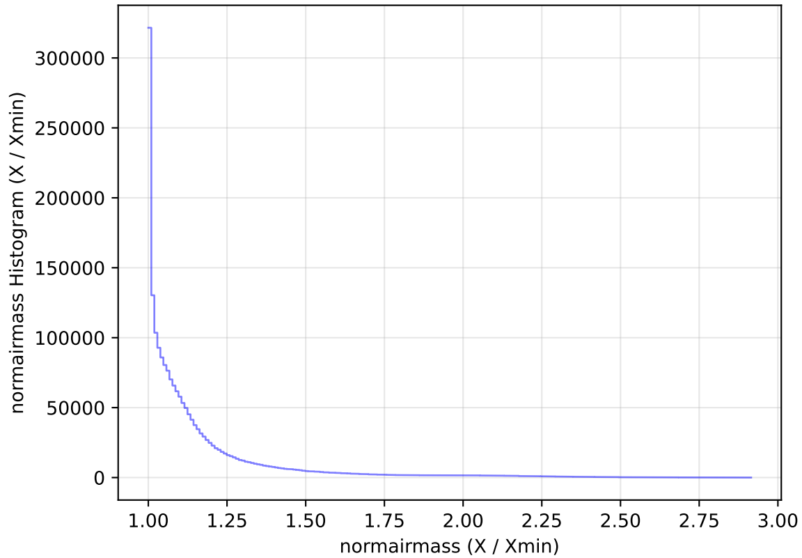
internal_u_expt60_nscale1.2v3.4_10yrs WFD all bands: normairmass Histogram
