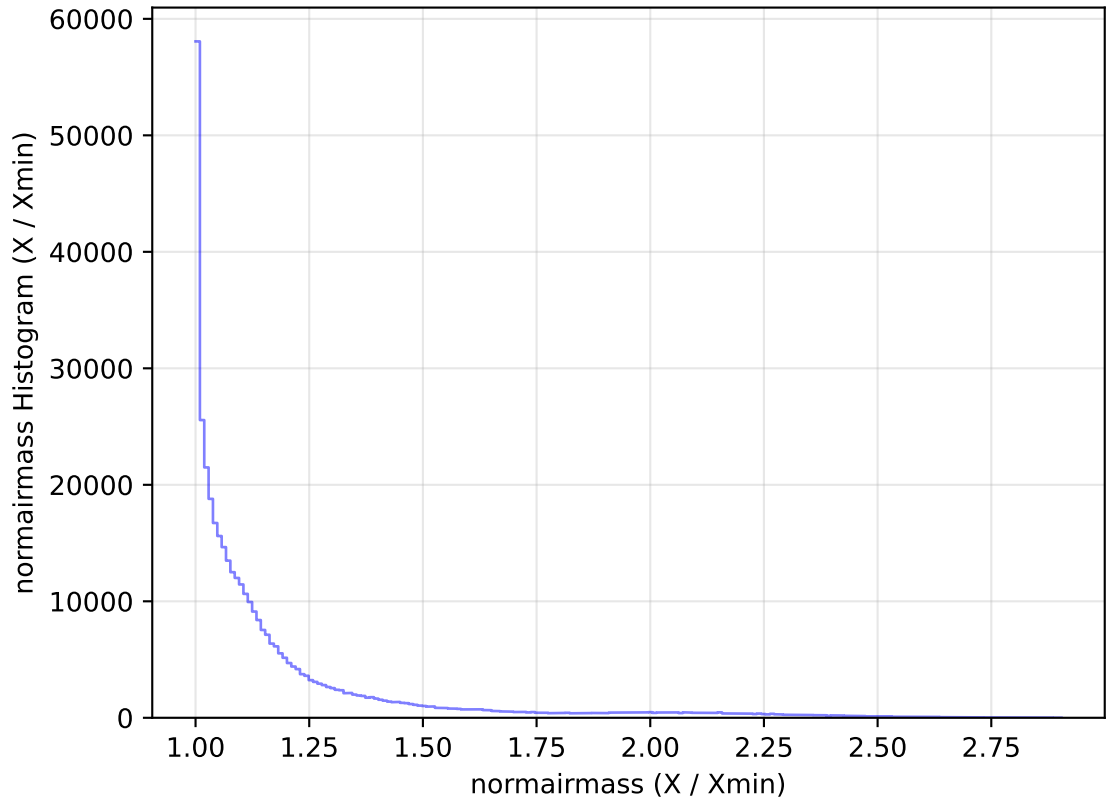
internal_u_expt60_nscale1.2v3.4_10yrs All sky z band: normairmass Histogram
