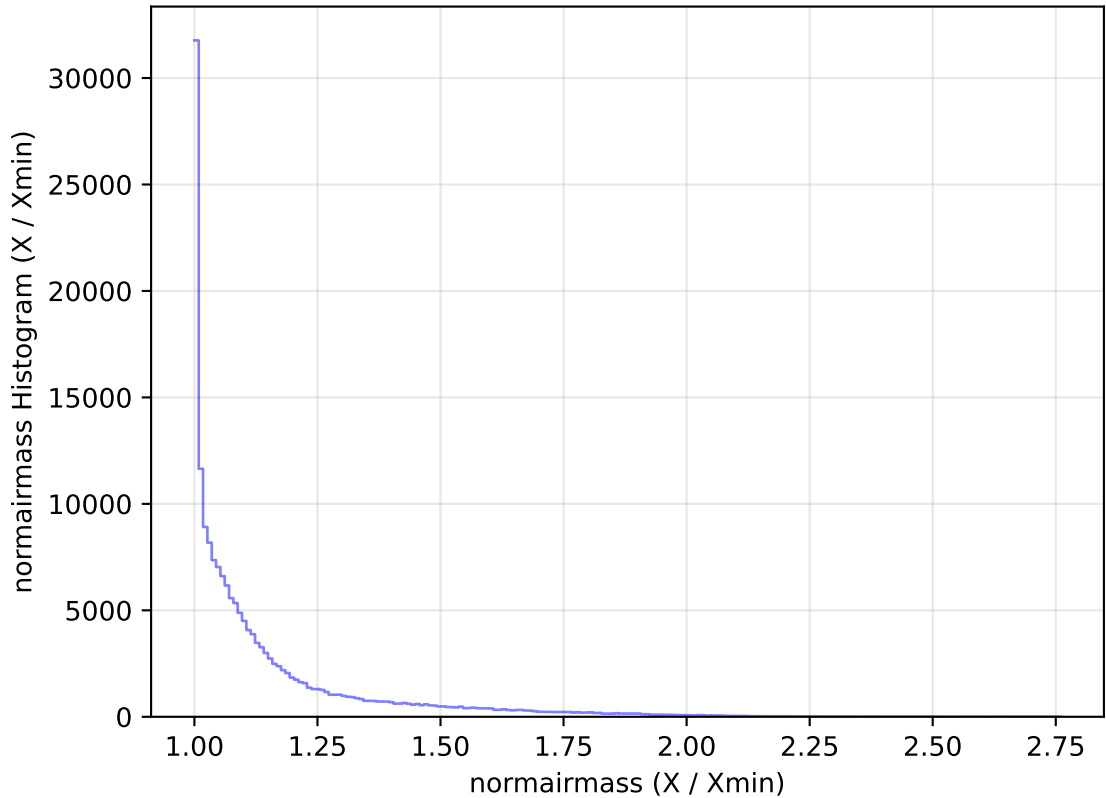
internal_u_expt60_nscale1.2v3.4_10yrs All sky g band: normairmass Histogram
