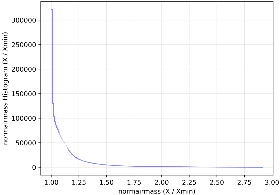
internal_u_expt60_nscale1.2v3.4_10yrs All sky all bands: normairmass Histogram
