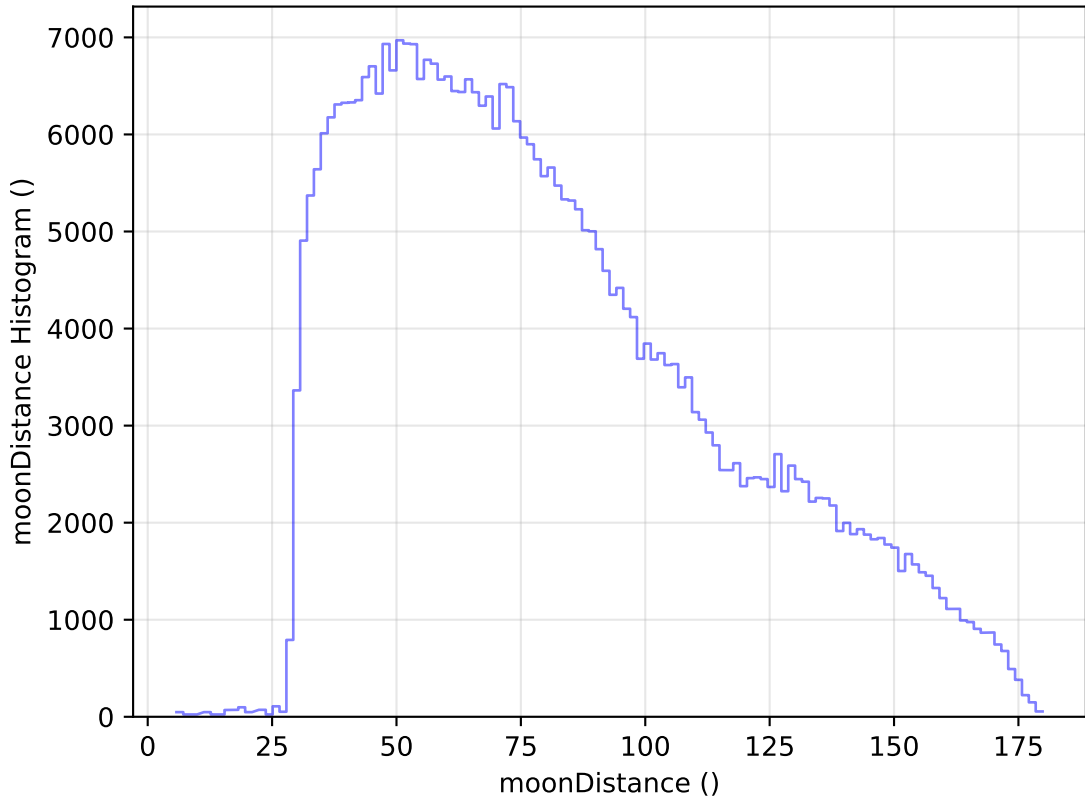
internal_u_expt60_nscale1.2v3.4_10yrs WFD z band: moonDistance Histogram
