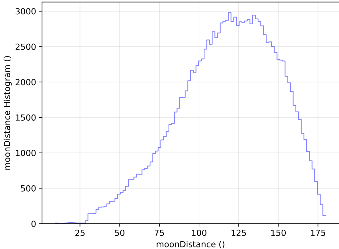
internal_u_expt60_nscale1.2v3.4_10yrs WFD u band: moonDistance Histogram
