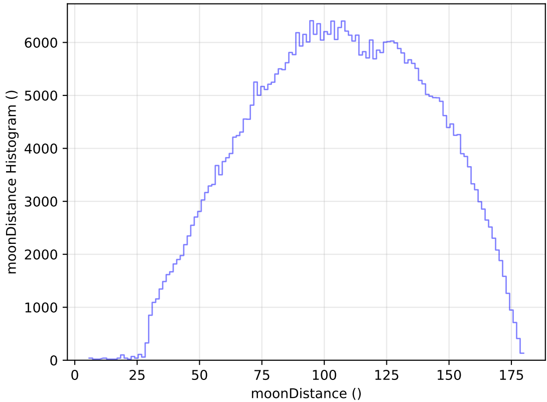
internal_u_expt60_nscale1.2v3.4_10yrs WFD r band: moonDistance Histogram
