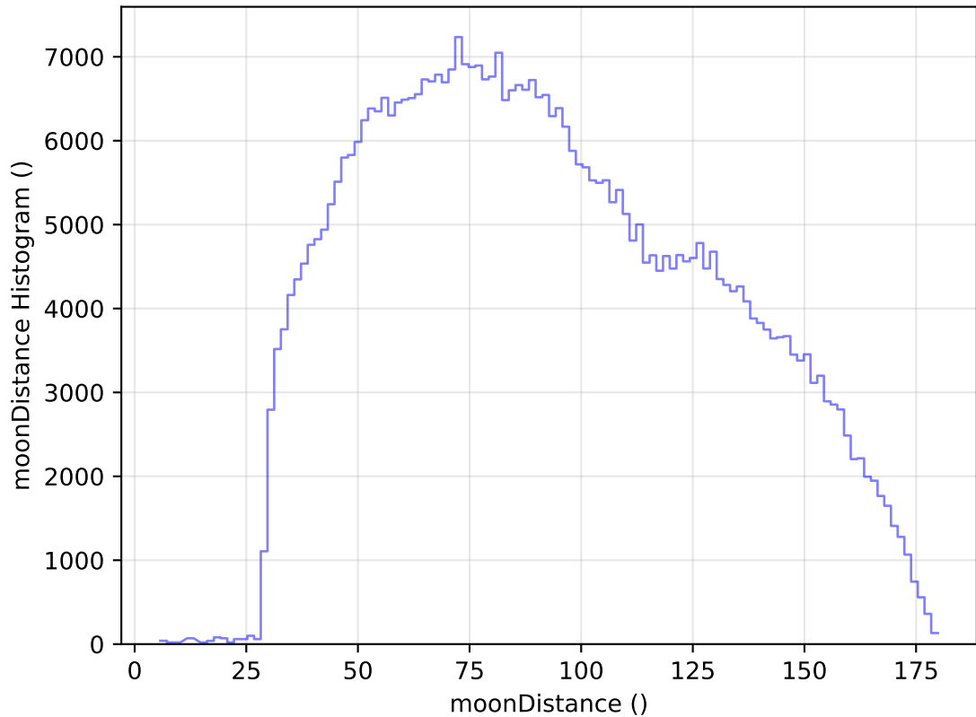
internal_u_expt60_nscale1.2v3.4_10yrs WFD i band: moonDistance Histogram
