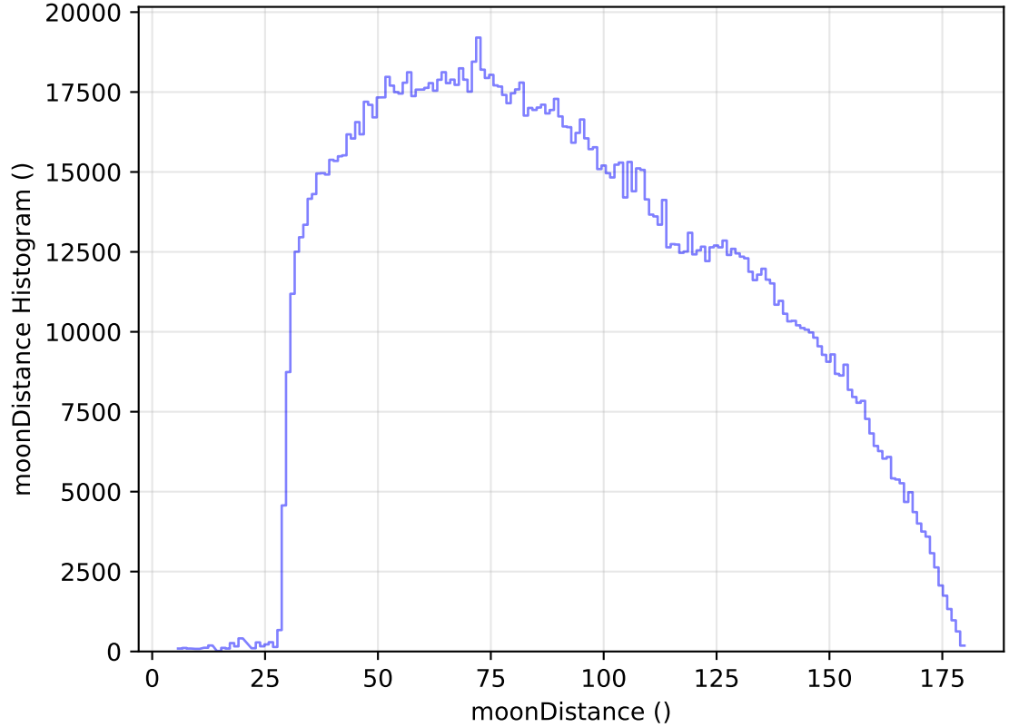
internal_u_expt60_nscale1.2v3.4_10yrs WFD all bands: moonDistance Histogram
