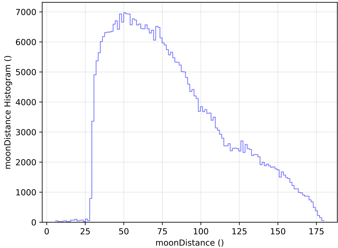
internal_u_expt60_nscale1.2v3.4_10yrs All sky z band: moonDistance Histogram
