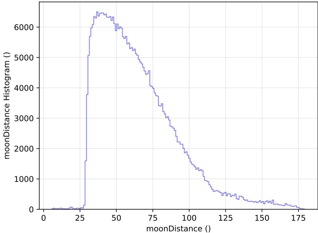
internal_u_expt60_nscale1.2v3.4_10yrs All sky y band: moonDistance Histogram
