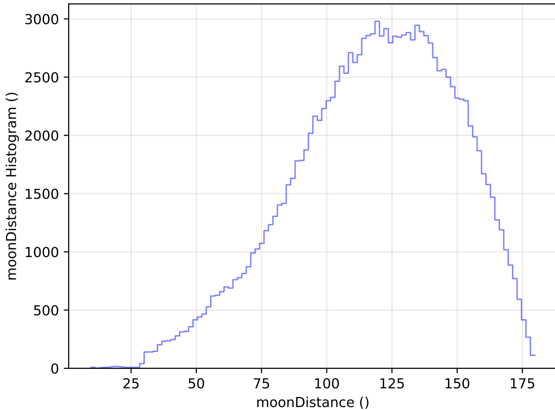
internal_u_expt60_nscale1.2v3.4_10yrs All sky u band: moonDistance Histogram
