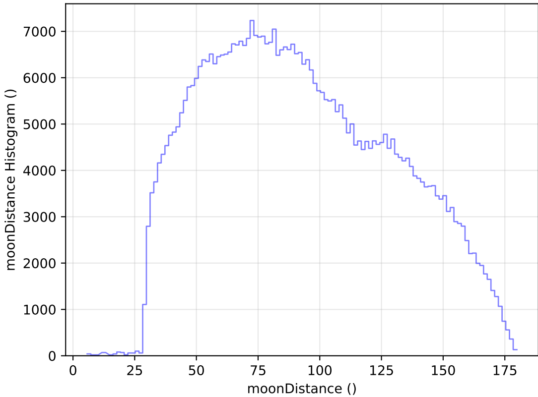
internal_u_expt60_nscale1.2v3.4_10yrs All sky i band: moonDistance Histogram
