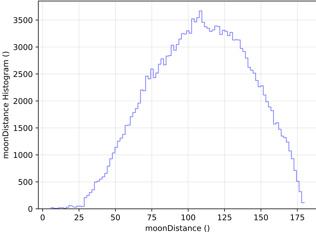
internal_u_expt60_nscale1.2v3.4_10yrs All sky g band: moonDistance Histogram
