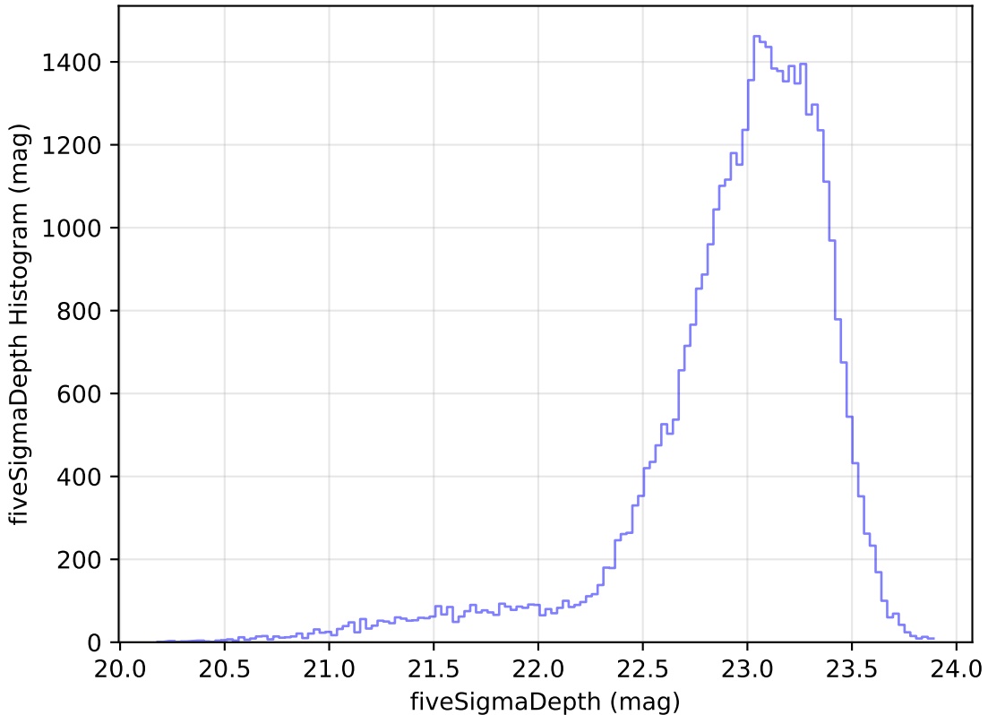
internal_u_expt60_nscale1.2v3.4_10yrs Yr 1 z band: fiveSigmaDepth Histogram
