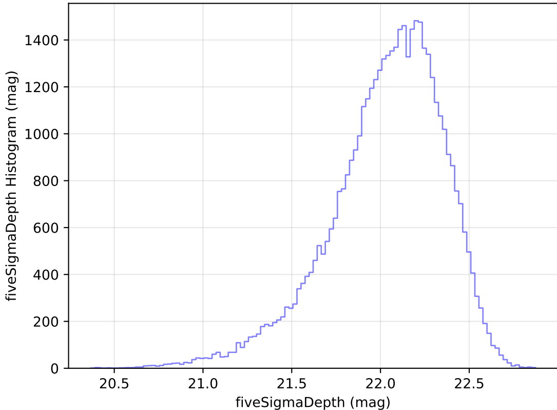
internal_u_expt60_nscale1.2v3.4_10yrs Yr 1 y band: fiveSigmaDepth Histogram
