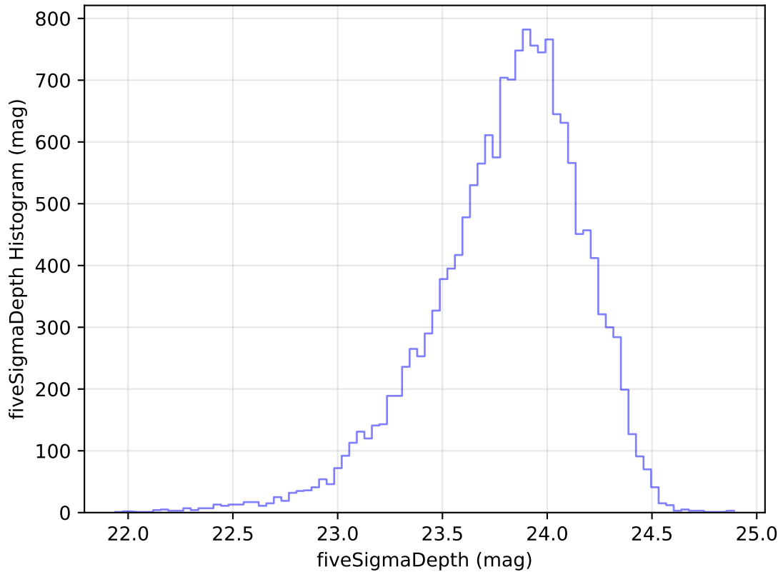
internal_u_expt60_nscale1.2v3.4_10yrs Yr 1 u band: fiveSigmaDepth Histogram
